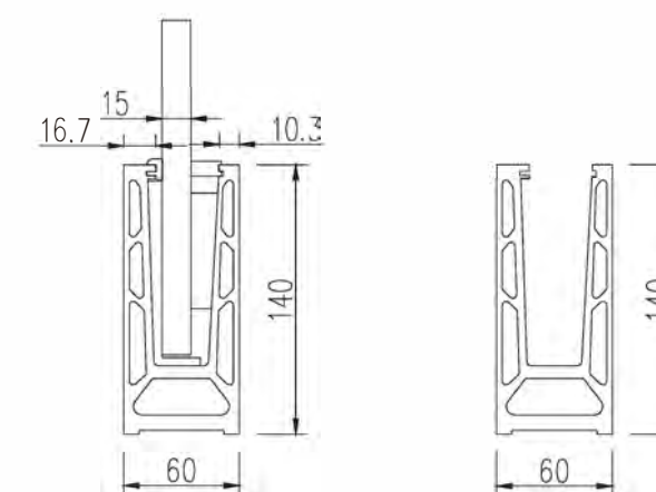
For 12mm to 19mm tempered glass
