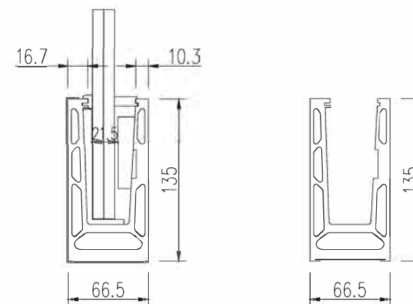
For 17mm to 24mm tempered glass
