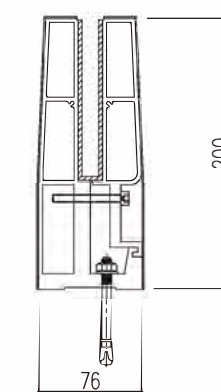
For 10mm to 15mm tempered glass
