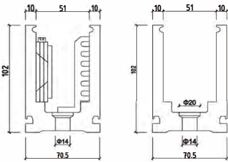
For Glass 19-24mm thick PAU 001-B
