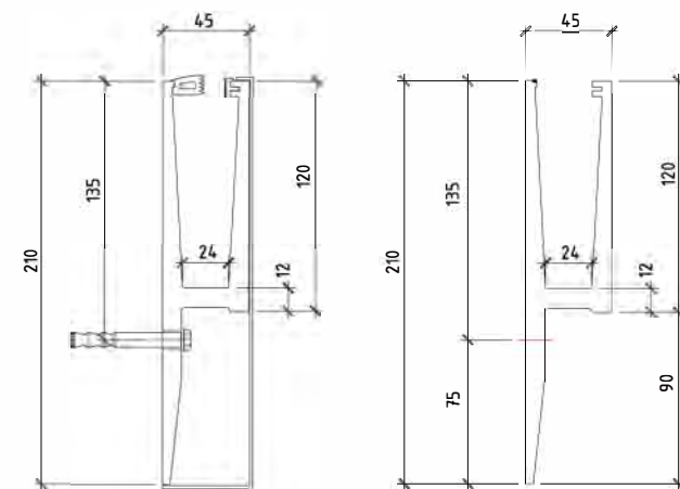
For 12mm to 6+1.52+6mm tempered laminated glass
