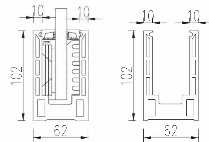
For 12mm to 15mm tempered glass
