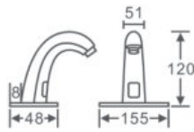
N-8008A / N-8008B Automatic sensor Faucet Metarial: Brass Color: Chrome
