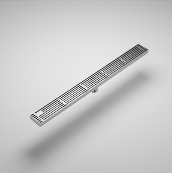
Floor drainer Size: 300x80mm/600x80mm (If want to customize length,need confirm with us) Material: 304 stainless steel Color: Brushed
