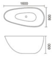
ON-1017 Free standing bathtub Material: Acrylic Size: 1300x720x600mm 1400x750x600mm 1500x800x600mm Size: 1600x800x600mm 1700x850x600mm Color: White/Black+White
