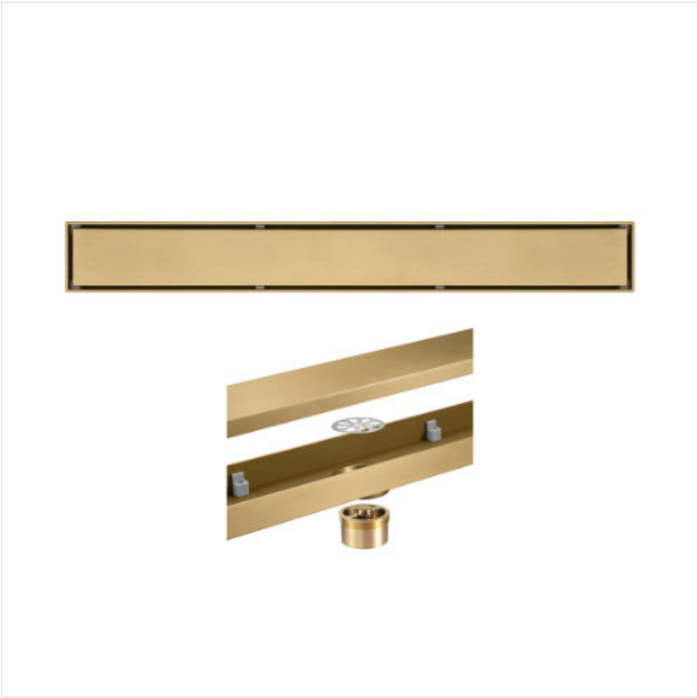
Size: 300x55mm/600x55mm/300x80mm/600x80mm (If want to customize length,need confirm with us) Material: 304 stainless steel Color: Brushed gold
