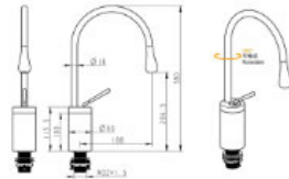
N-8001A / N-8001B Automatic sensor Faucet Metarial: Brass Color: Chrome
