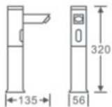
N-8022A / N-8022B Automatic sensor Faucet Metarial: Brass Color: Chrome
