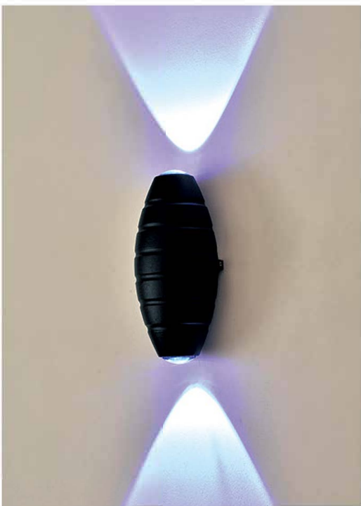
GMD-F861 Lamp: LED 2 x 3W Size: 160 x 70 x 60
