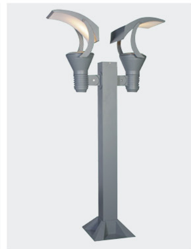
GMD-2088B-2 E27 × 2/PAR30 LED:(12 × 1W) × 2 Size:Φ165 × H1000mm
