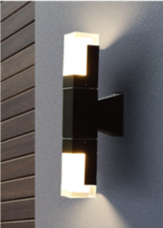
GMD-900-2 Lamp:LED 2 × 3W Size:65 × 65 × 350
