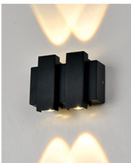
GMD-F815B-2 Lamp:LED 4 × 1W Size:120 × 90 × 42
