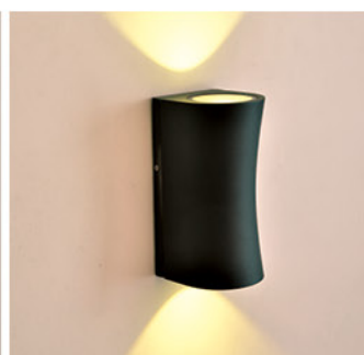
GMD-F810 Lamp:LED 2 × 7W Size:200 × 100 × 100
