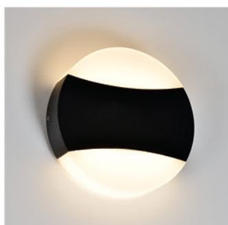
GMD-F880 Lamp:LED 2 × 6W Size:Φ 160 × 35
