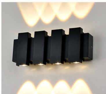
GMD-F815B-4 Lamp:LED 8 × 1W Size:220 × 90 × 42
