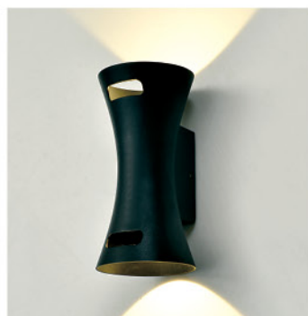
GMD-F859 Lamp: LED 2 × 5W Size: 200 × 100 × 107
