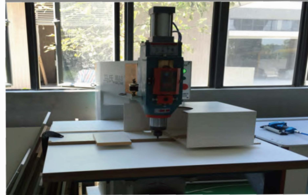
CNC Router
